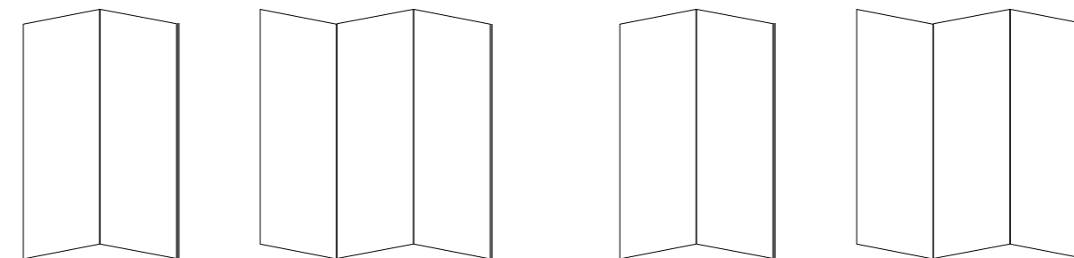
QUINTA F158X300 L 140 (70+70) H 198 cm QUINTA F159X450 L 210 (70+70+70) H 198 cm QUINTA SOUND F160X350 L 128 (64+64) H 198 cm QUINTA SOUND F161X480 L 192 (64+64+64) H 198 cm
